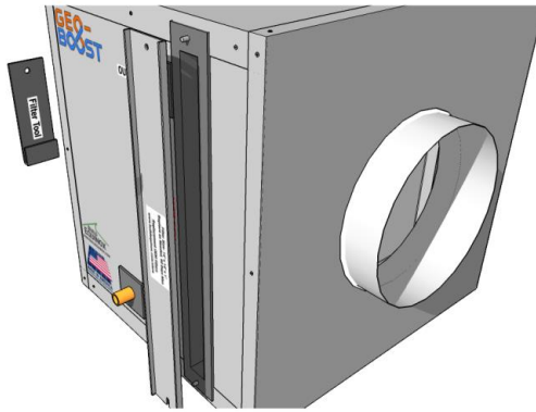
Remove filter access panel and set aside
